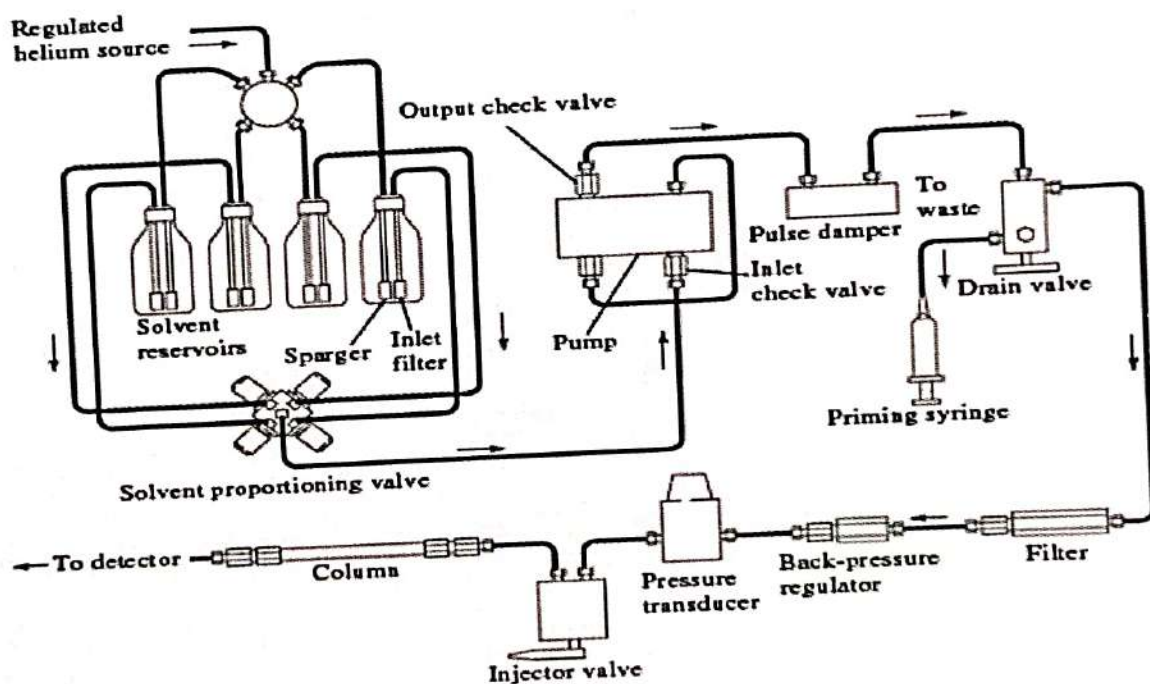
FLOW CHART SHOWING TYPICAL COMPONENTS OF HPLC
